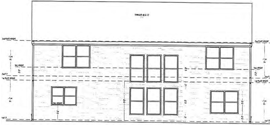
REAR ELEVATION SCALE: 1/8" = 1'-0" SUB CONDITION SHOWN
