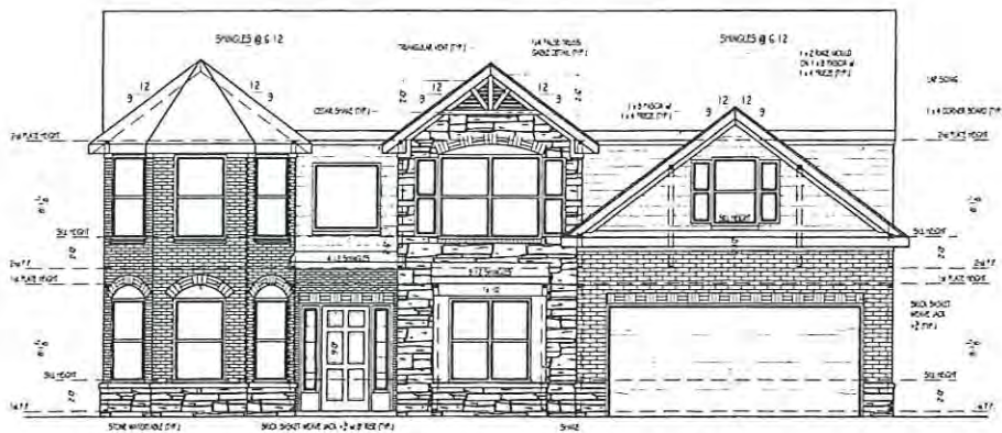
FRONT ELEVATION C7
