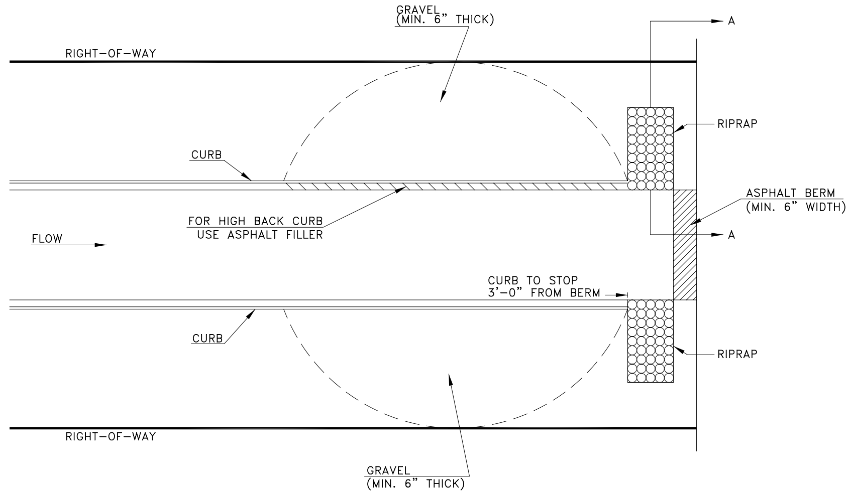
PLAN
