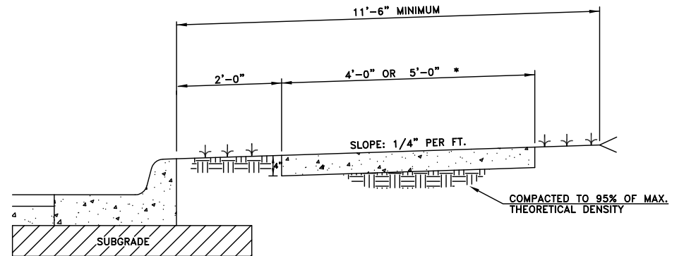
TYPICAL SECTION OF SIDEWALK
