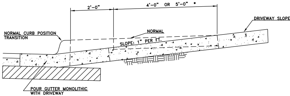
SIDEWALK SECTION AT DRIVEWAY
