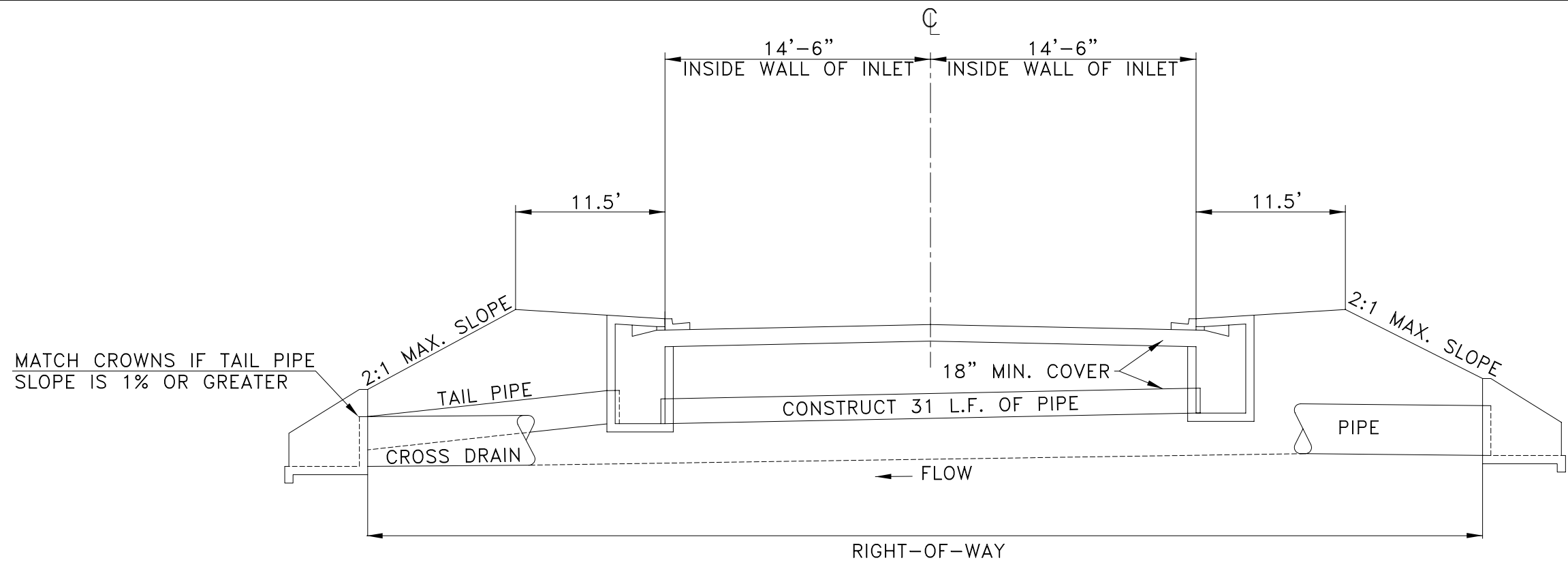
SECTION
