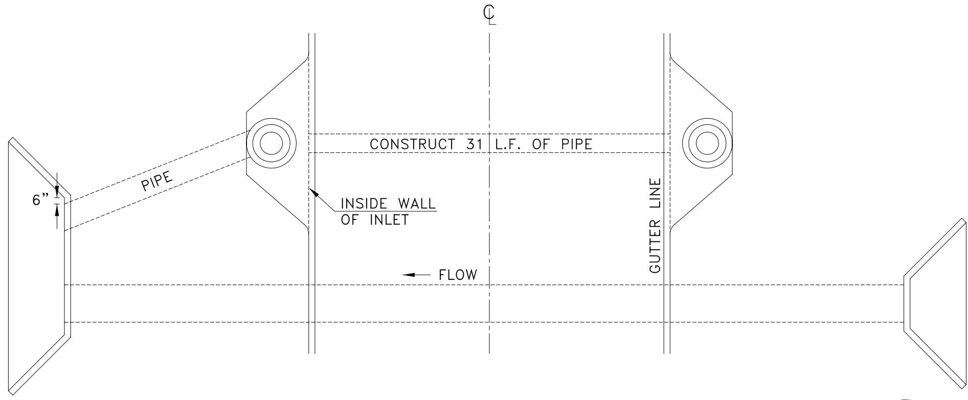
PLAN
