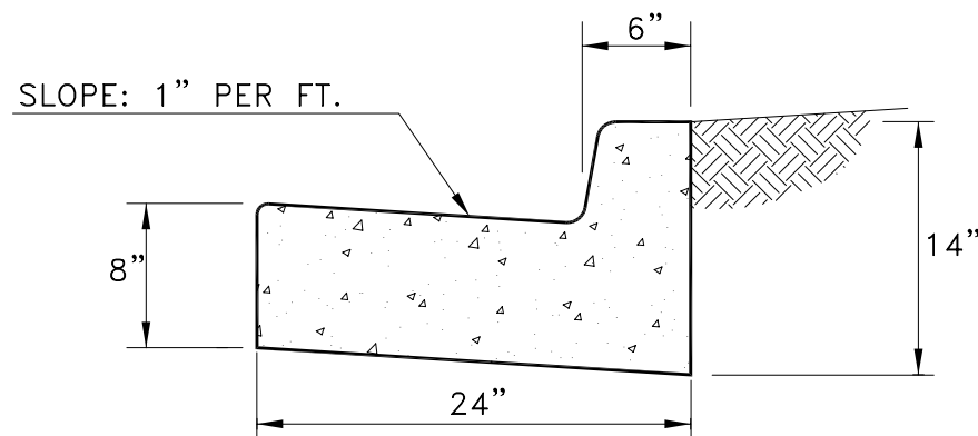
SECTION B-B 24" VERTICAL CURB AND GUTTER (COMMERCIAL AND INDUSTRIAL)
