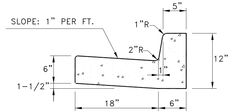
SECTION B-B 24" VERTICAL CURB AND GUTTER (RESIDENTIAL)
