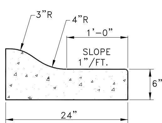
SECTION A-A ROLLED TYPE CURB AND GUTTER (WAIVER REQUIRED)
