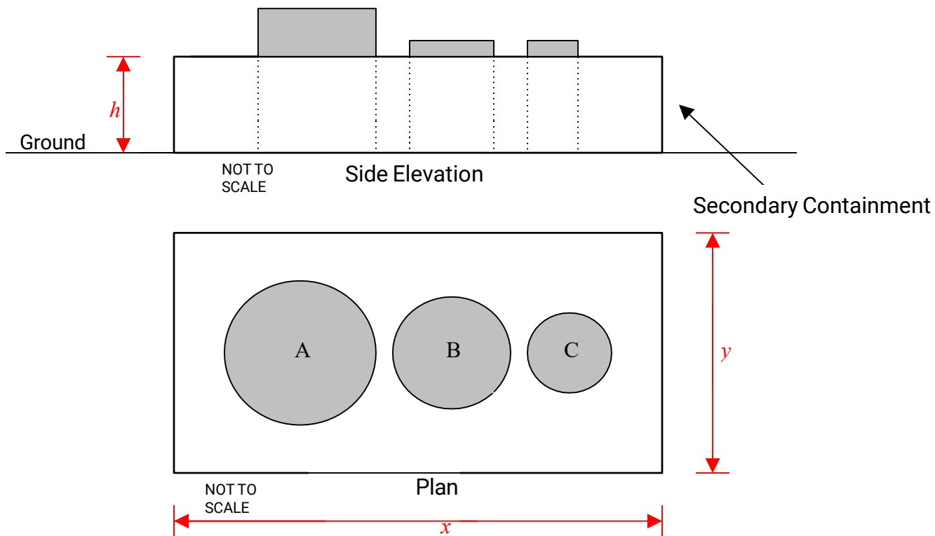
Figure 2 Example Calculations for Secondary Containment Storage Capacity
