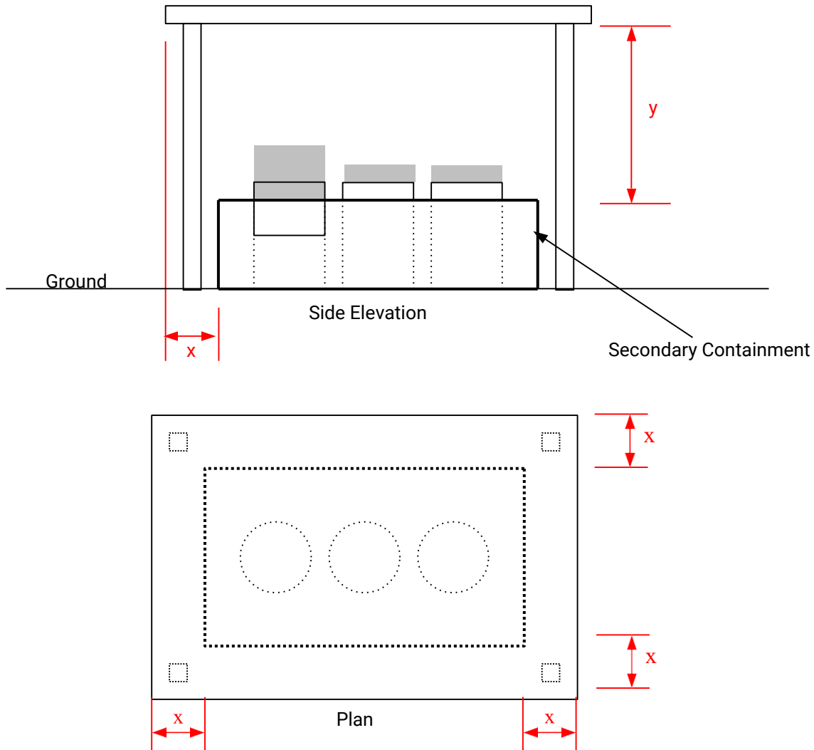
Figure 1 Secondary Containment Cover Overhang Detail
