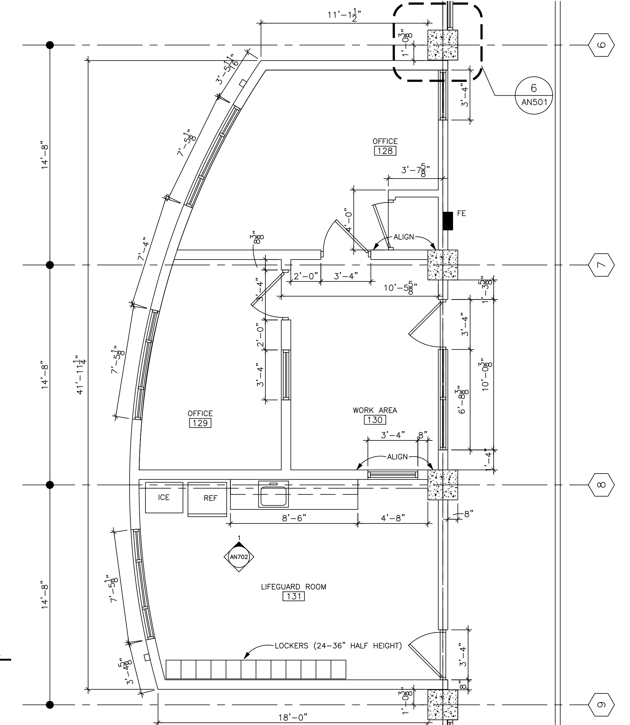
2 ENLARGED PLAN - OFFICE AREA 1/4" = 1'-0"
