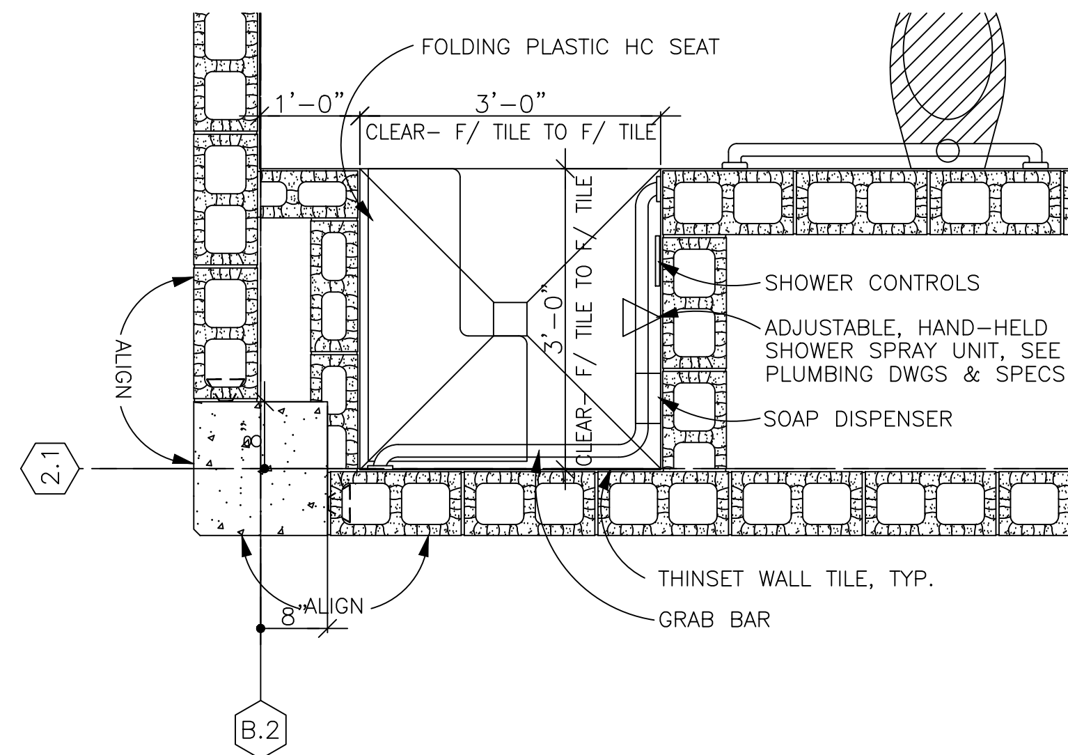
3 ENLARGED PLAN - HC SHOWER 3/4" = 1'-0"
