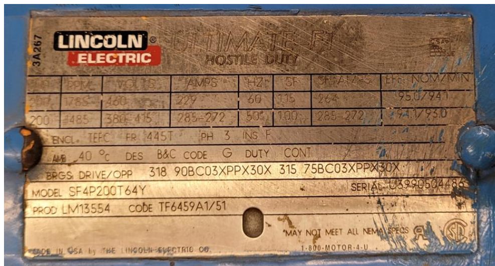
Photo 1 of 1: (Existing Motors -Nameplate) Typical of 2
